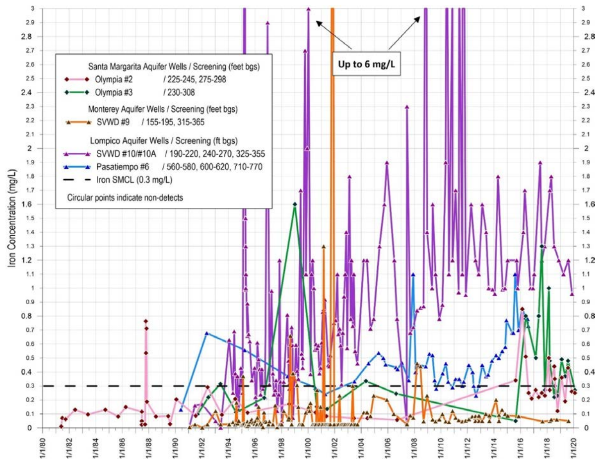
Figure 2-57. Iron Concentrations in Select Wells from 1980-2019
