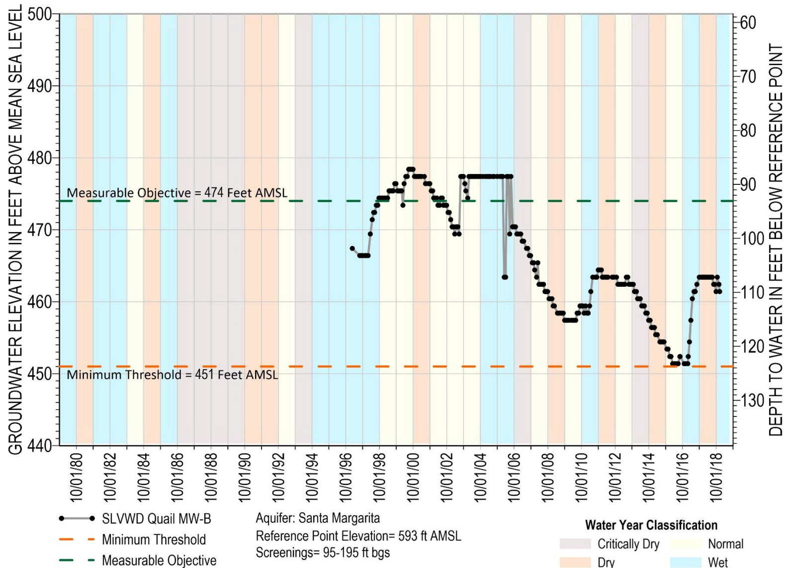
Figure 3-14: Hydrograph for SLVWD Quail MW-B in the Santa Margarita Aquifer Showing Minimum Threshold and Measurable Objective Relative to Measured Groundwater Elevations
