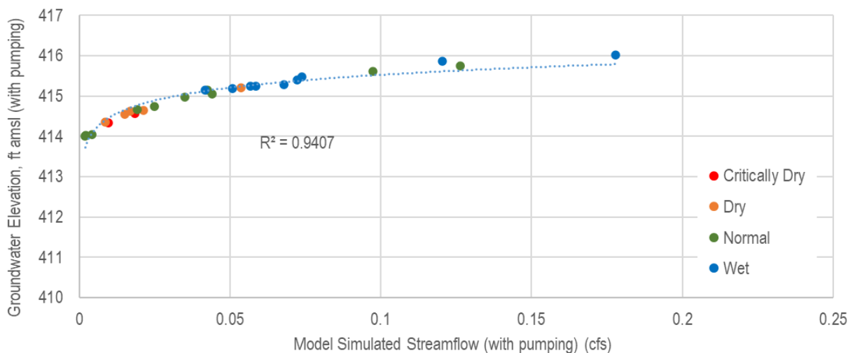
Figure 3-18. SLVWD Quail MW-A September Model Simulated Streamflow Compared to Groundwater Elevations
