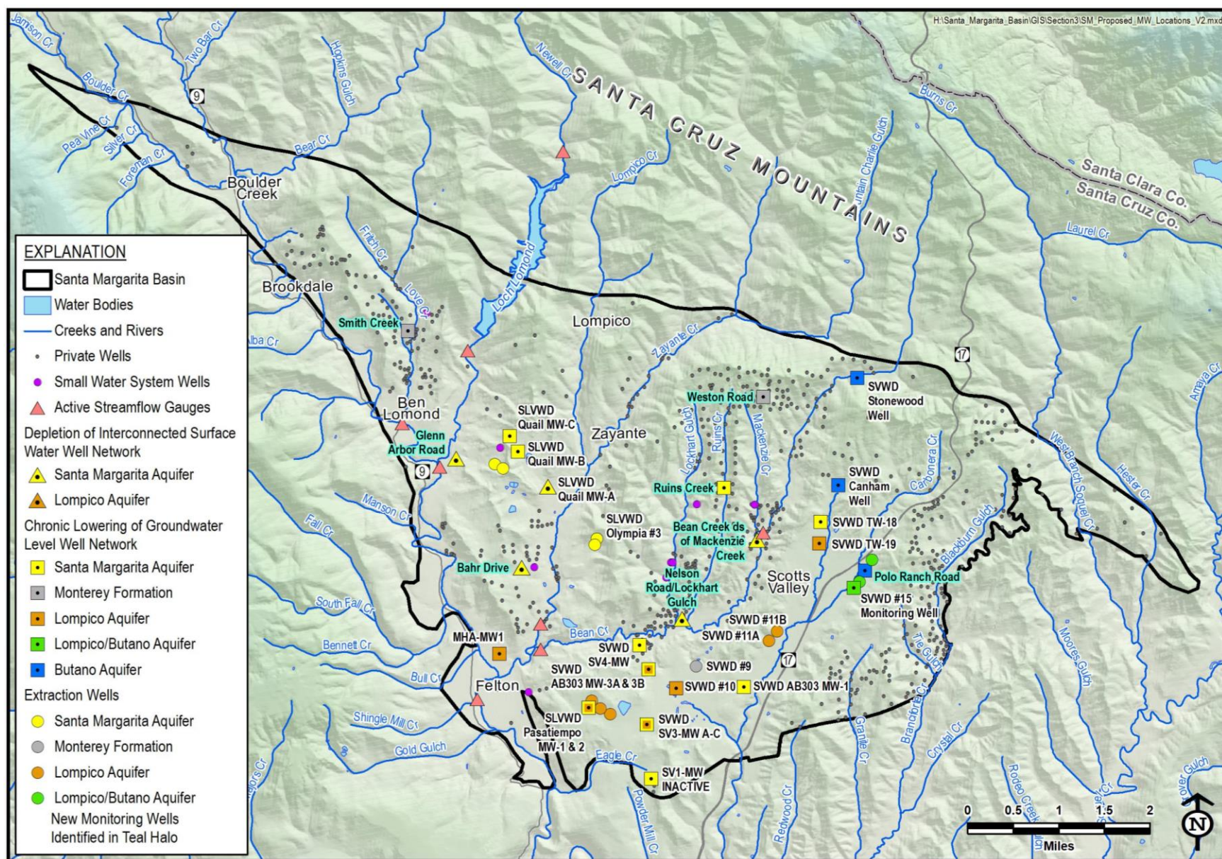
Figure 3-6. New Monitoring Wells (Teal Label) in Relation to Existing Monitoring Features
